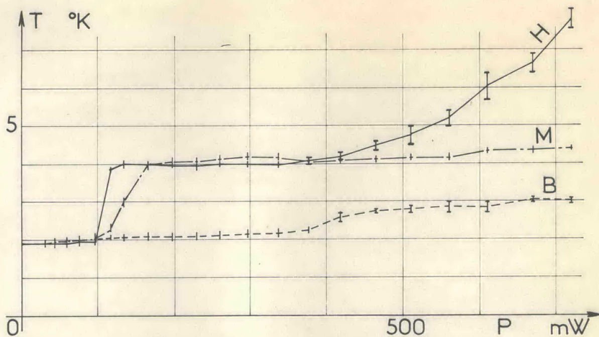
FIG.11 : Superfluid helium T = 1.9 K ; p = 1 atm
